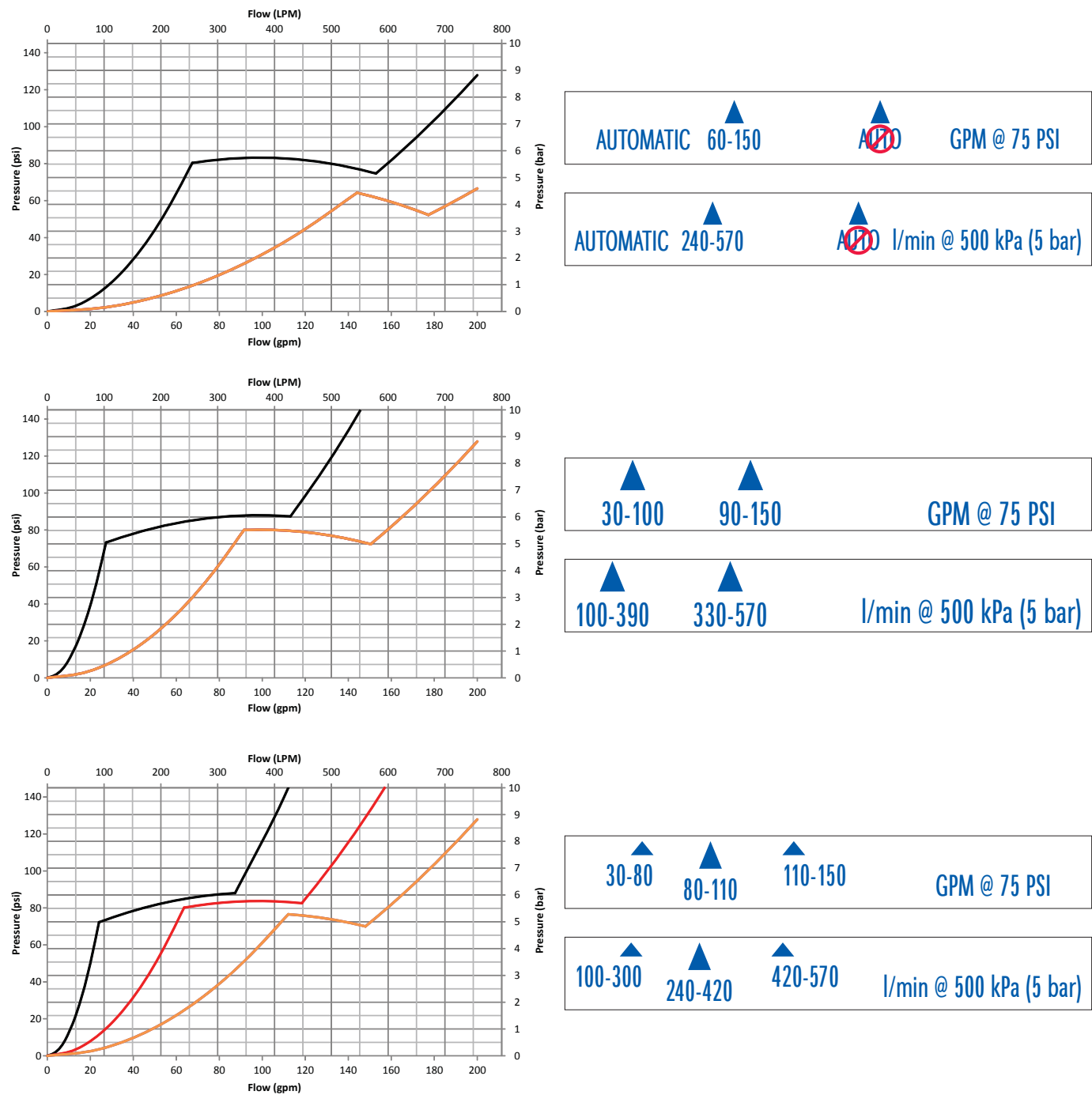
Figure 4.4A G-Force Automatic With Flow Limiting
