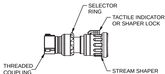
TIP ONLY NOZZLE
