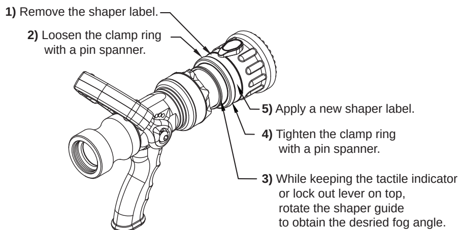
Figure 5.2.4A Flash over adjustment
