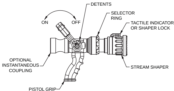
NOZZLE WITH VALVE & INTEGRAL PISTOL GRIP
