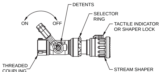
NOZZLE WITH VALVE
